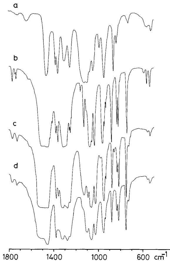
Fig. 4. Typical IR. spectra of complexes with 15-crown-5 ( 1 ). (a) Ligand alone, (b) \text{Pr}(\text{NO}_3)_3 \cdot \mathbf{1} , (c) \text{Ho}(\text{NO}_3)_3 \cdot \mathbf{1} , and (d) [\text{Ho}(\text{NO}_3)_3]_4 \cdot (\mathbf{1})_3 .
